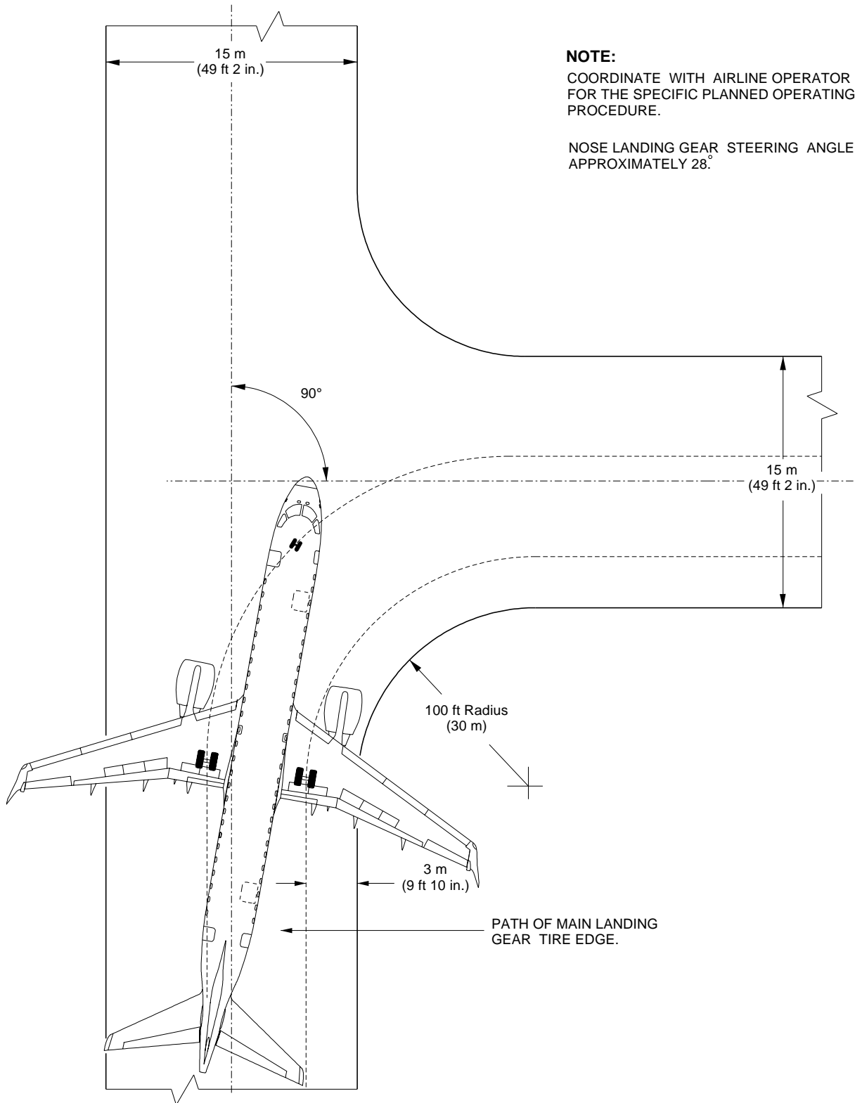
90° Turn - Taxiway to Taxiway Figure 4.8
