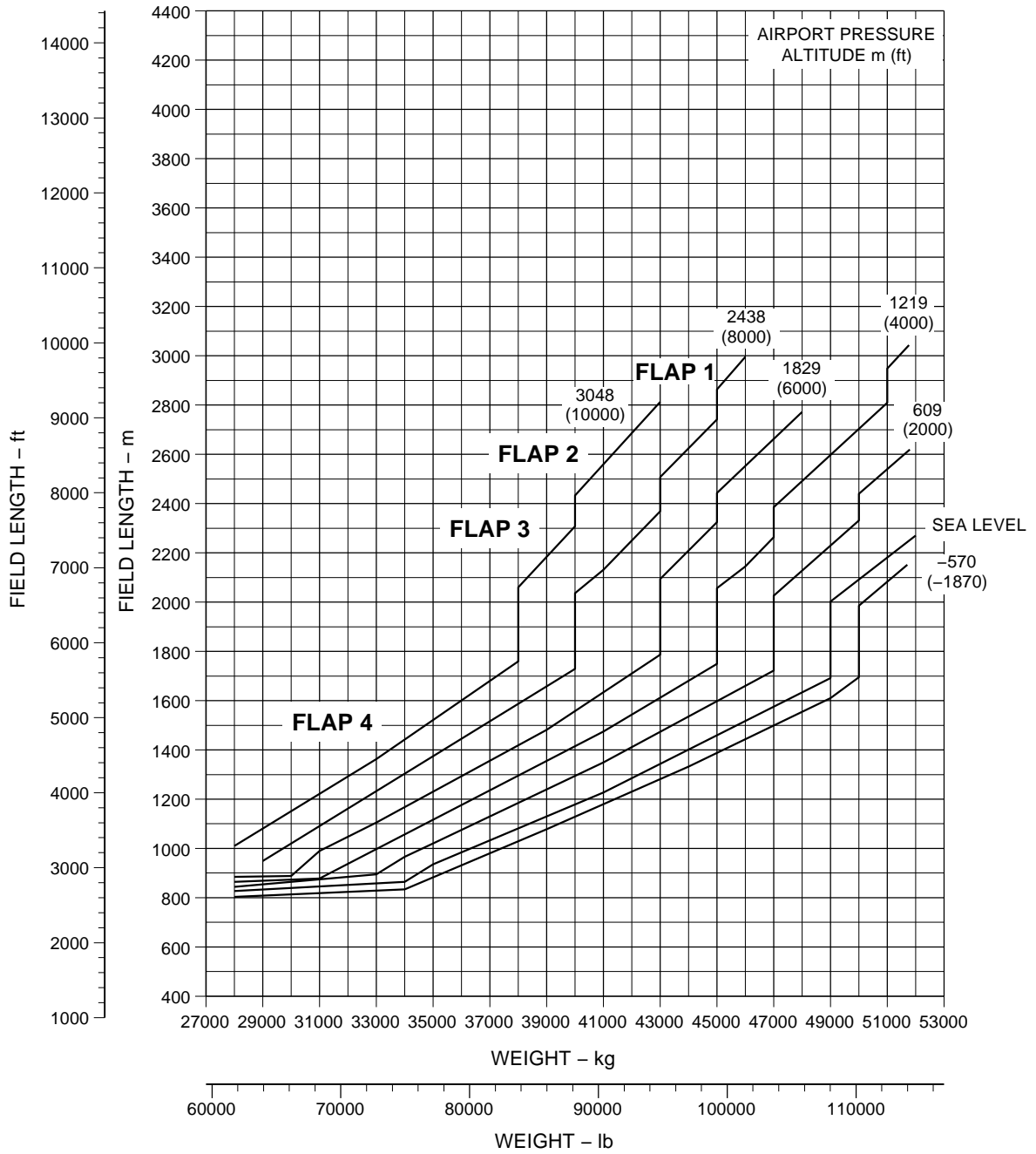
Takeoff Field Lengths - ISA + 15 °C Conditions Figure 3.16
