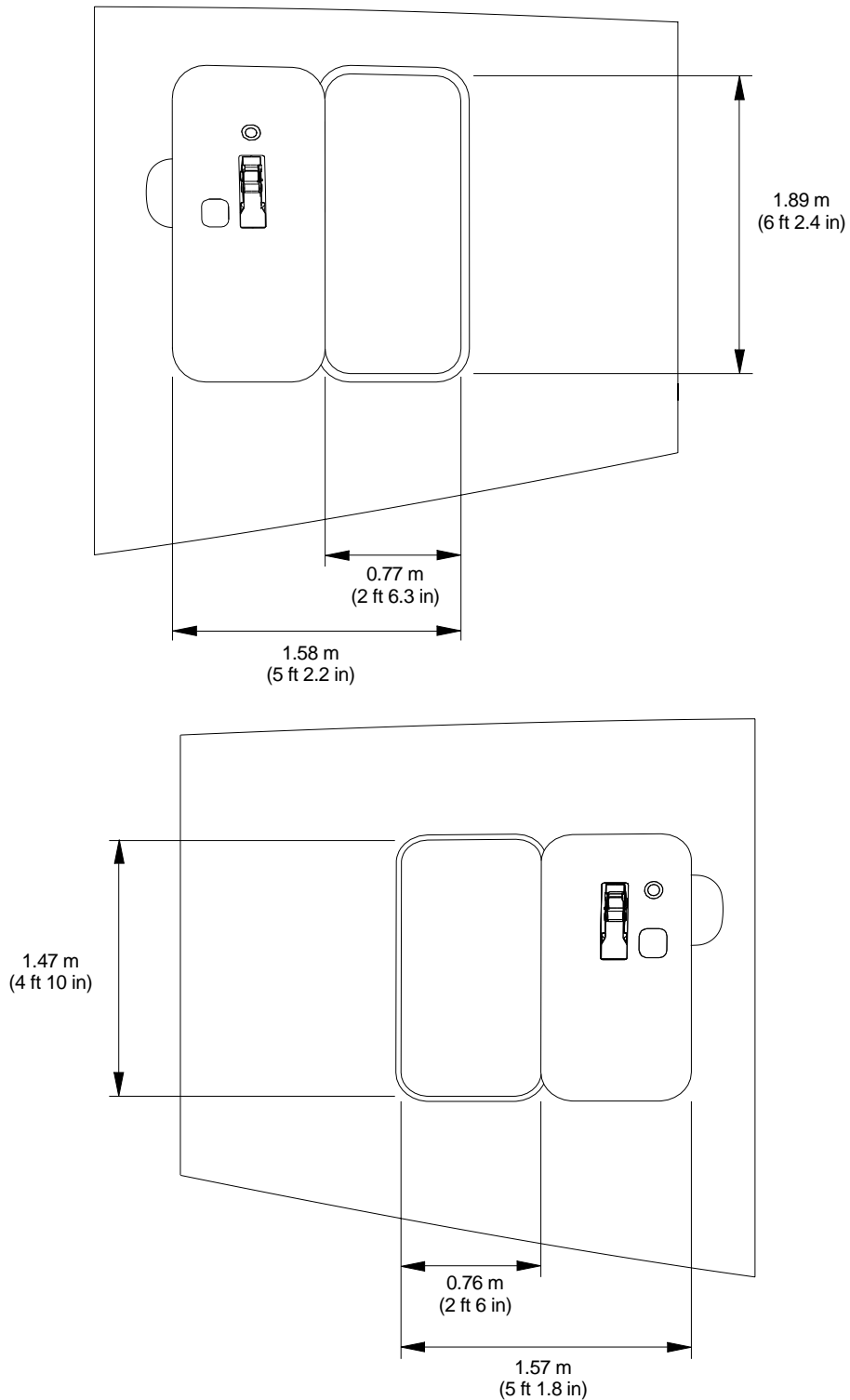
Passenger and Service Doors Dimensions Figure 2.2 Sheet 2
