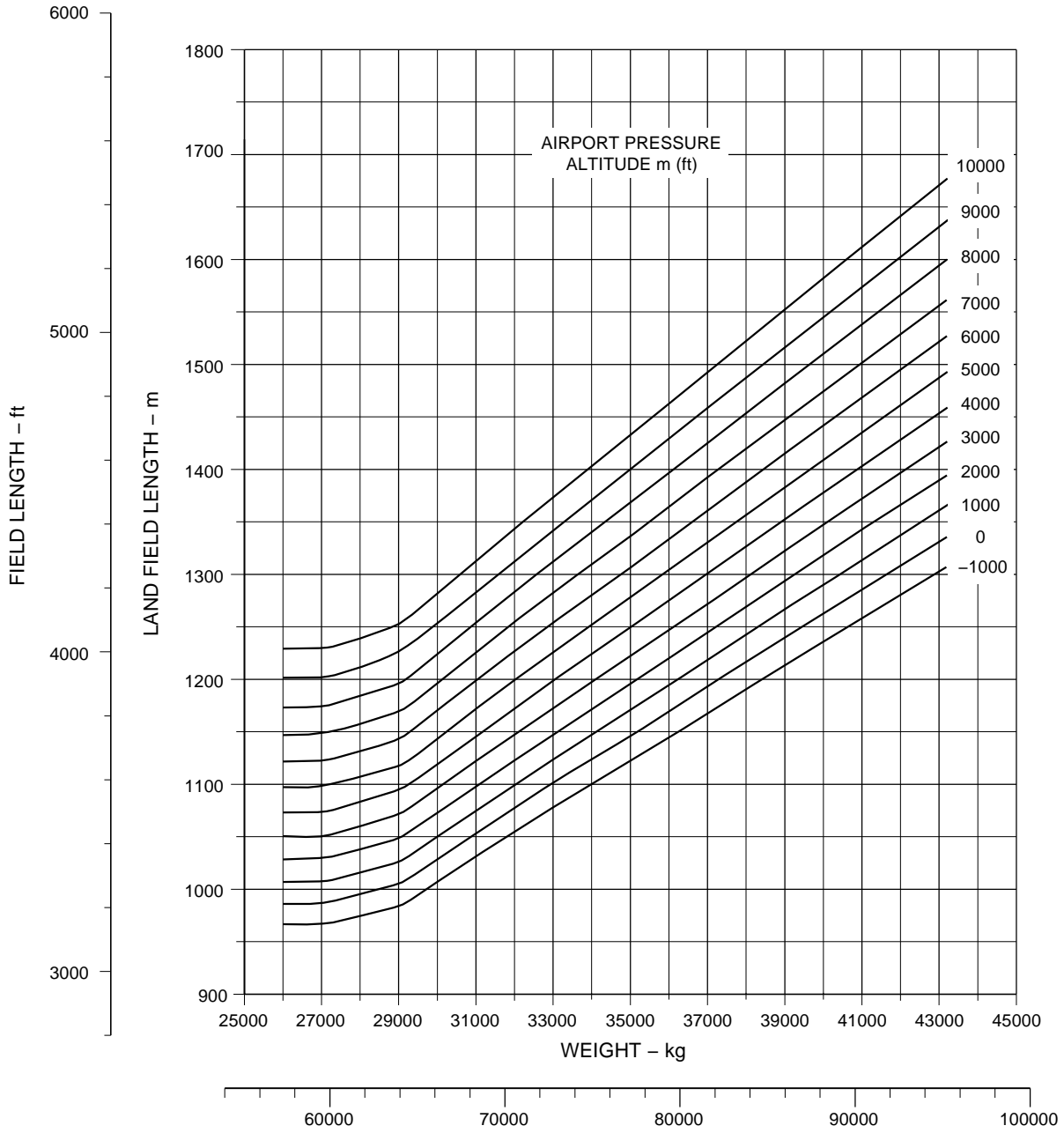
Landing Field Lengths - Flaps 5 Figure 3.17
