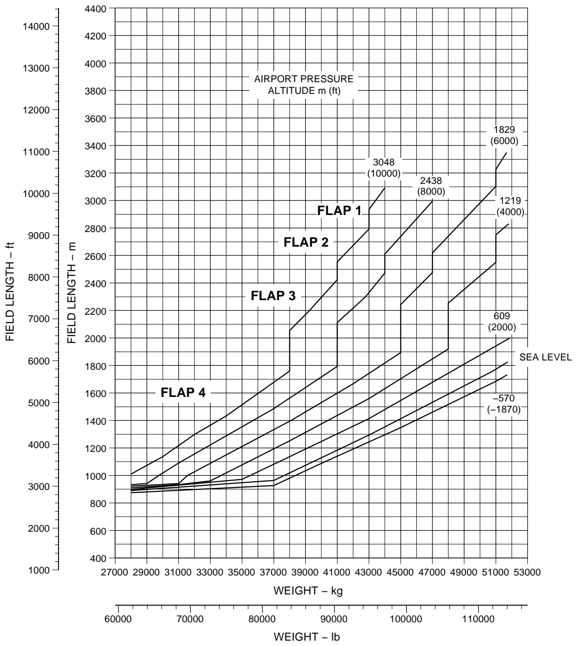
Takeoff Field Lengths - ISA + 15 °C Conditions Figure 3.14
