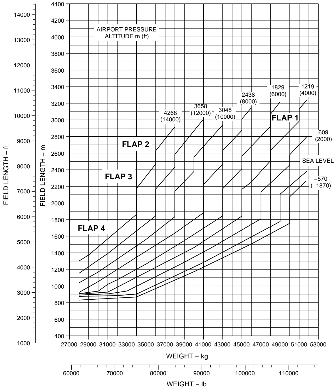
Takeoff Field Lengths - ISA + 15 °C Conditions Figure 3.10
