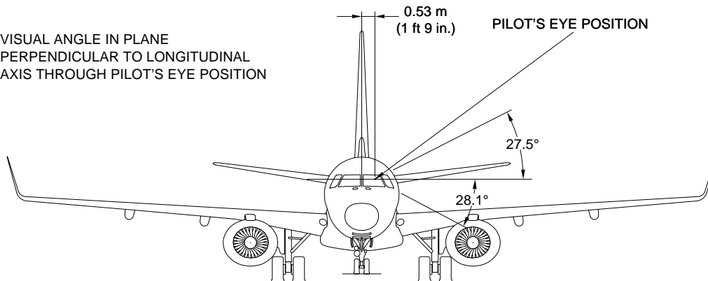
Visibility from Cockpit in Static Position Figure 4.3
