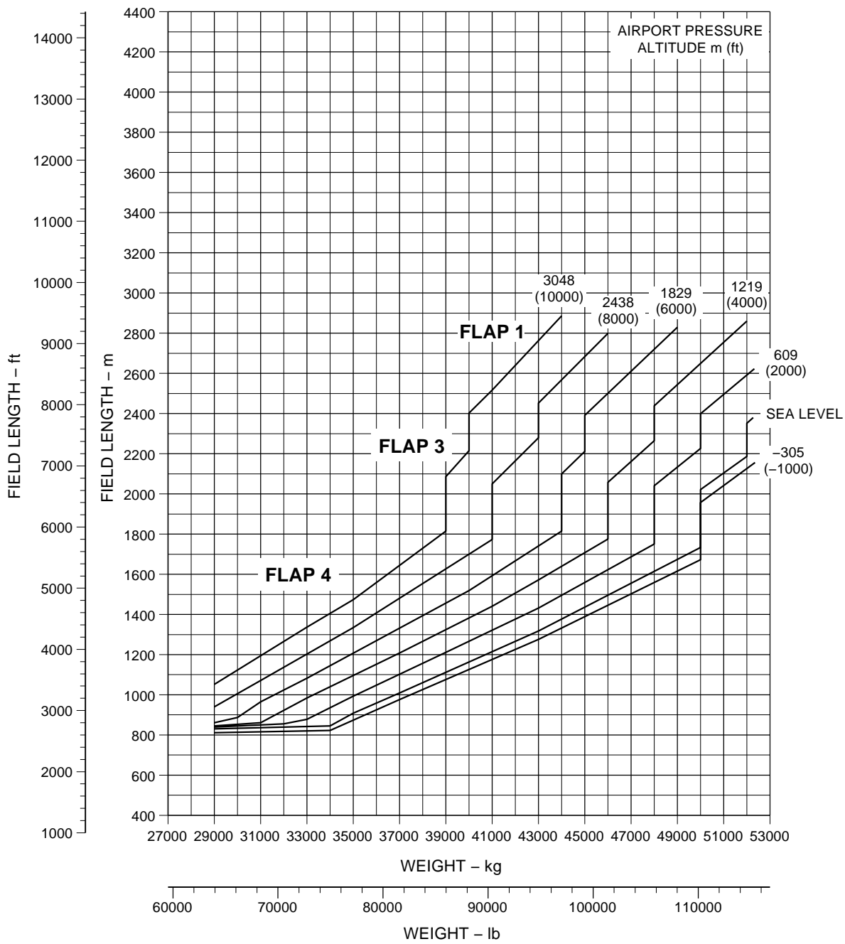
Payload x Range - ISA Conditions Figure 3.7
