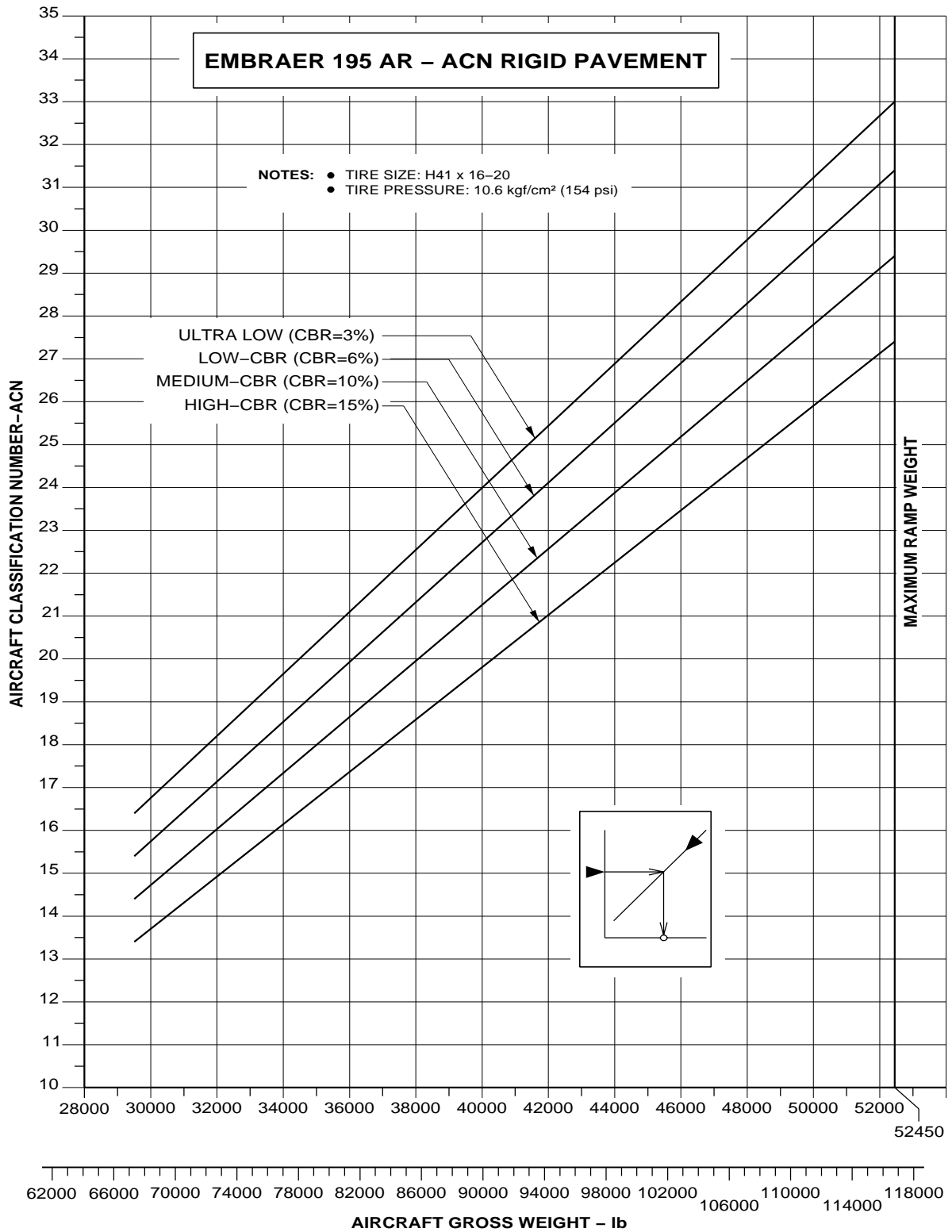
ACN For Rigid Pavement Figure 7.13
