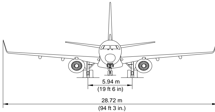
General Aircraft Dimensions Figure 2.1
