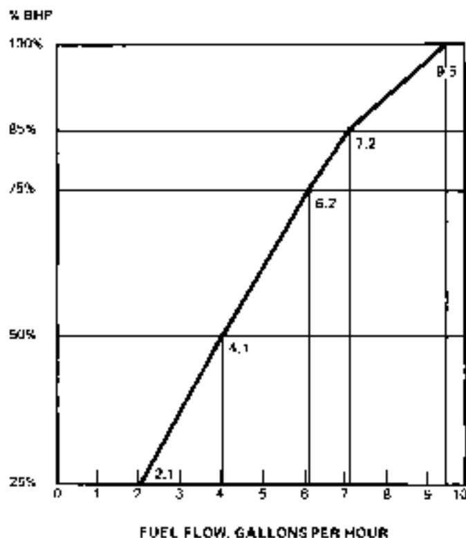
Figure A-4 Fuel Flow Chart
