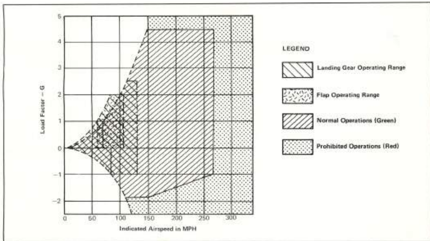
Figure 5-2 VN Diagram
