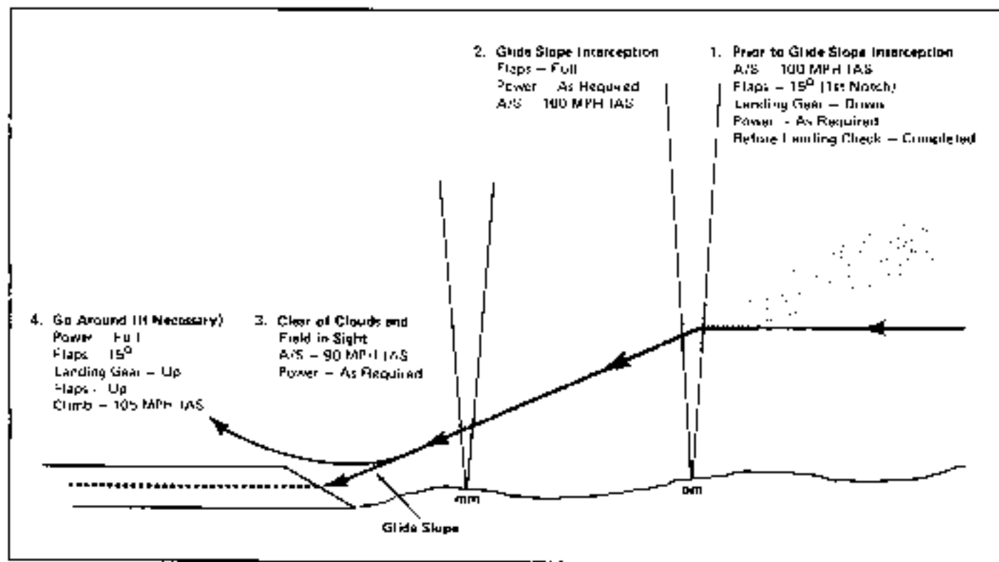
Figure 8-3 ILS Approach
