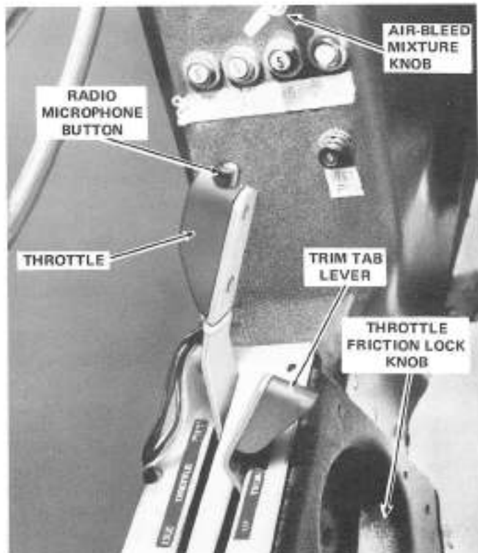
Figure 1-1 Left Console
