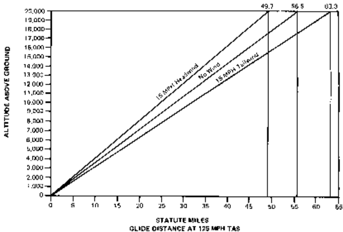
Figure 3-1 Glide Distance Chart
