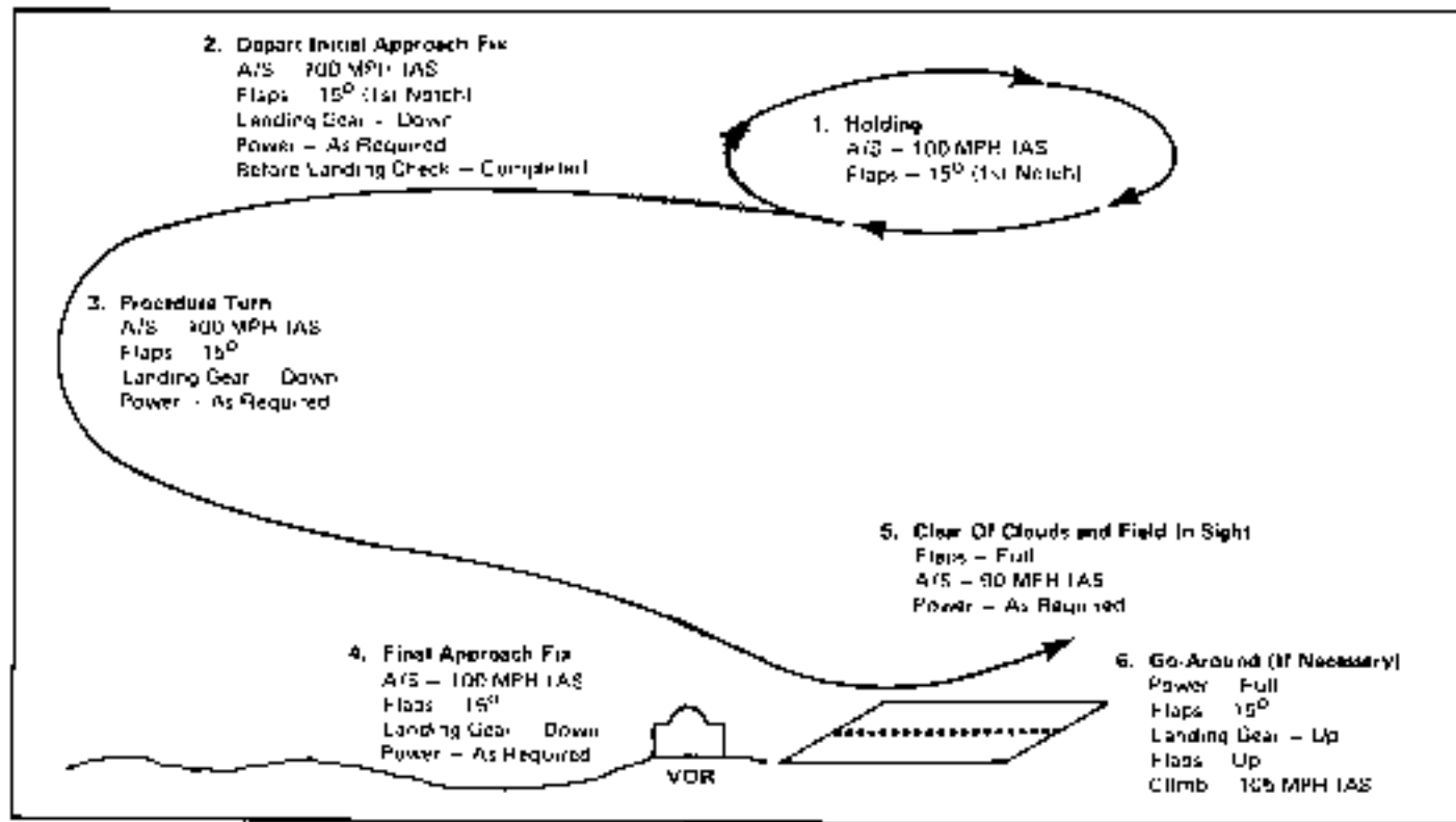
Figure B-1 VOR Approach
