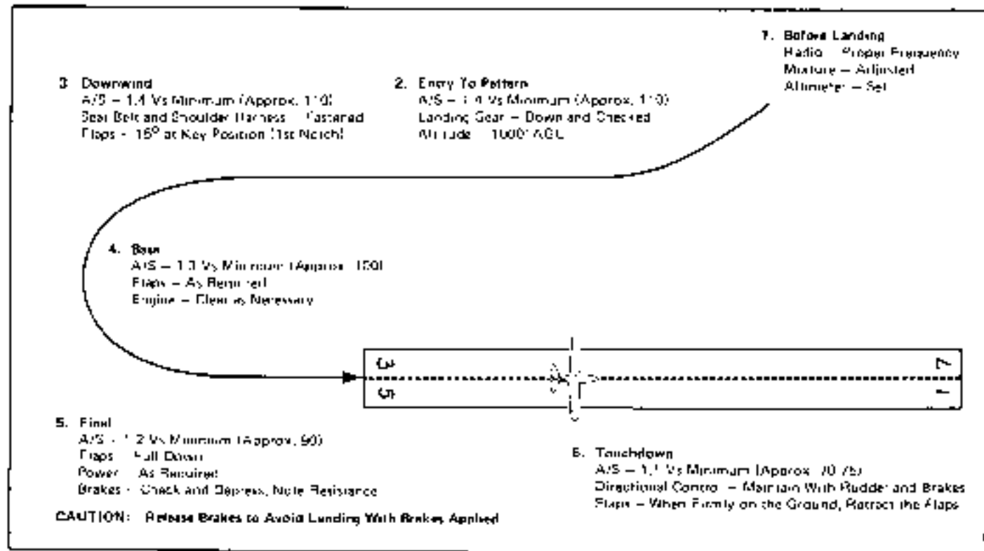
Figure 2-2 Diagram of Normal Landing Pattern
