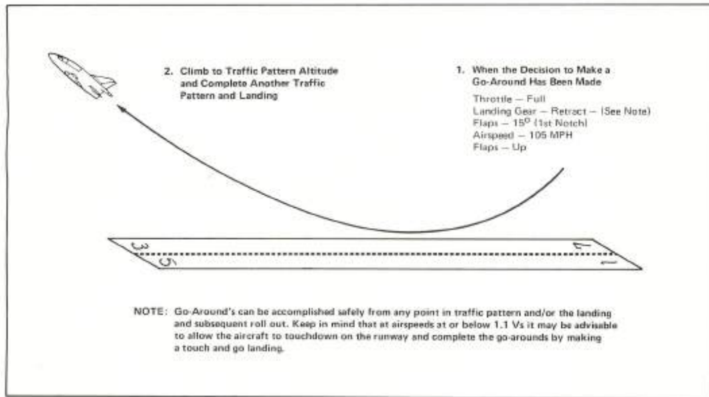
Figure 2-3 Diagram of Go-Around
