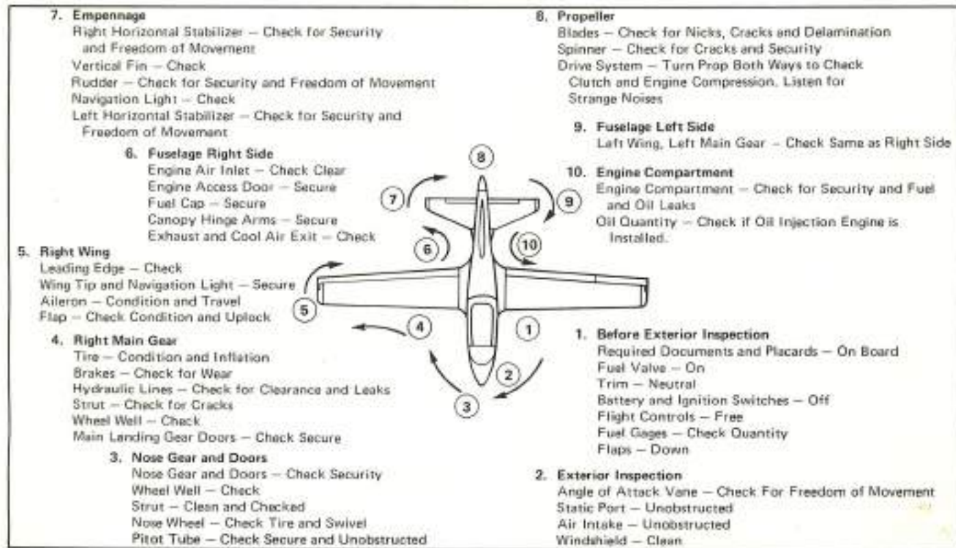
Figure 2-1 Diagram of Preflight Inspection Route
