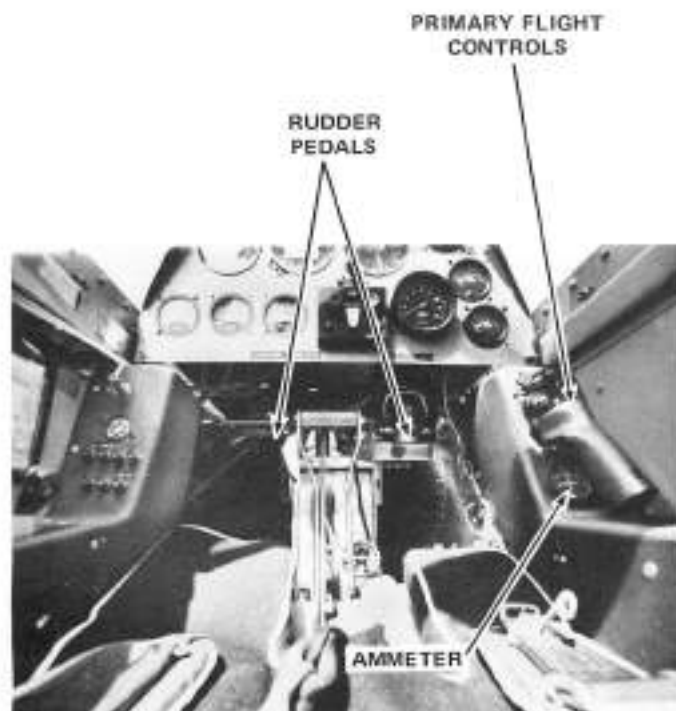
Figure 1-6 Rudder Pedals
