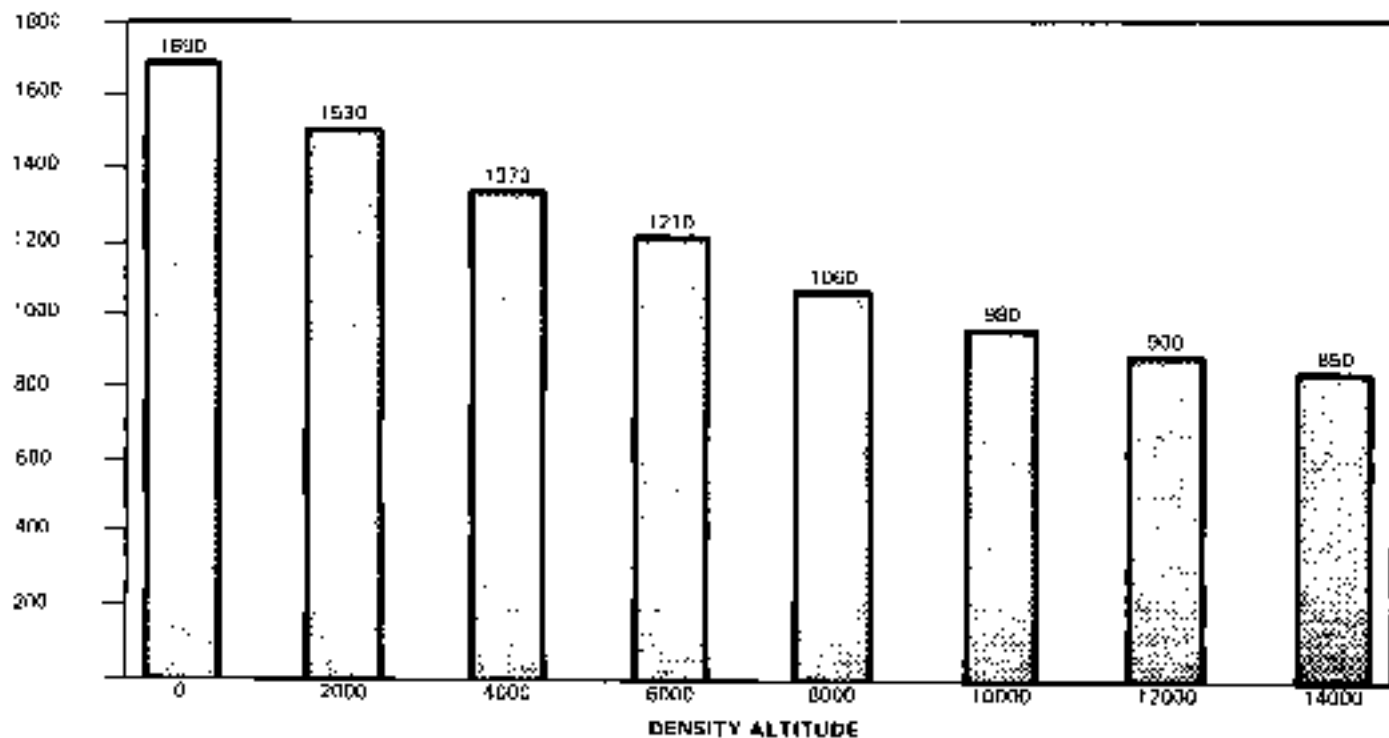
Figure A-8 Rate of Climb Chart
