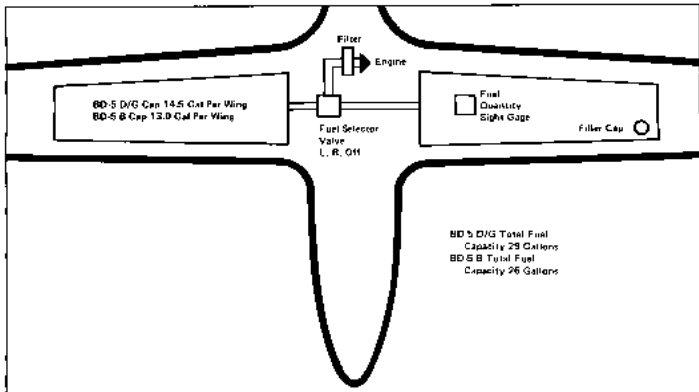
Figure 1-6 Fuel System
