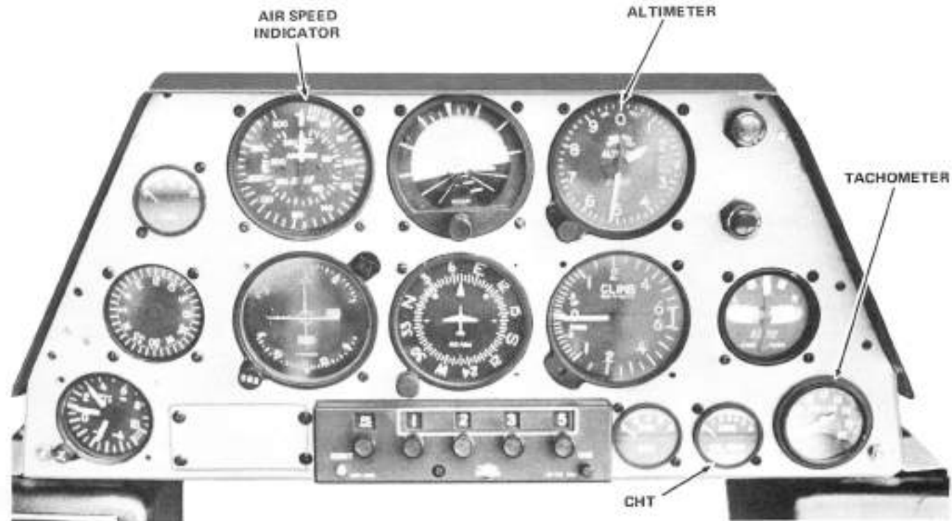
Figure 1-2 Instrument Panel
