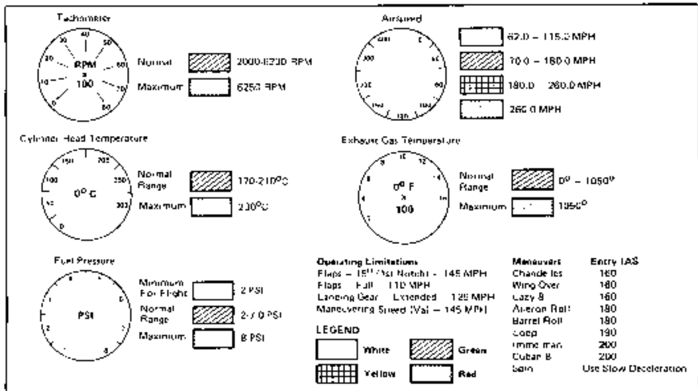
Figure 5-1 Instruments Markings and Operating Limitations Placard
