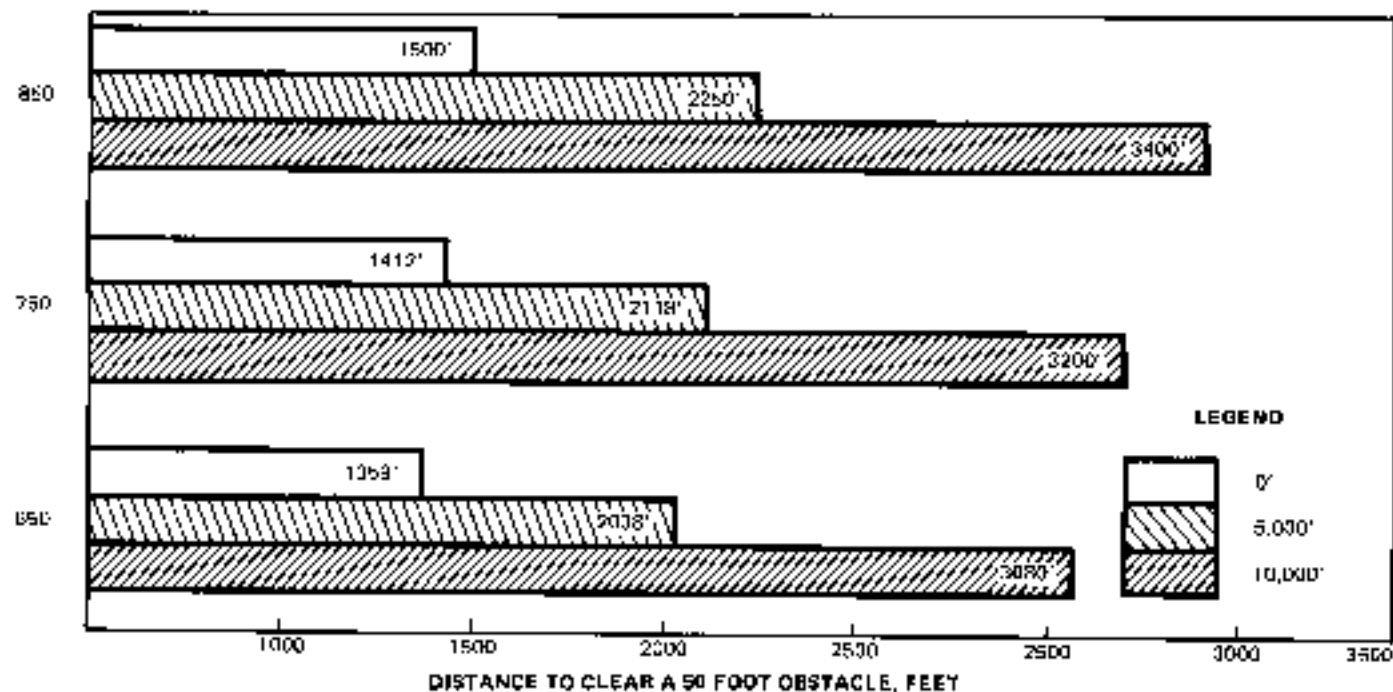
Figure A-5 Takeoff Distance Chart
