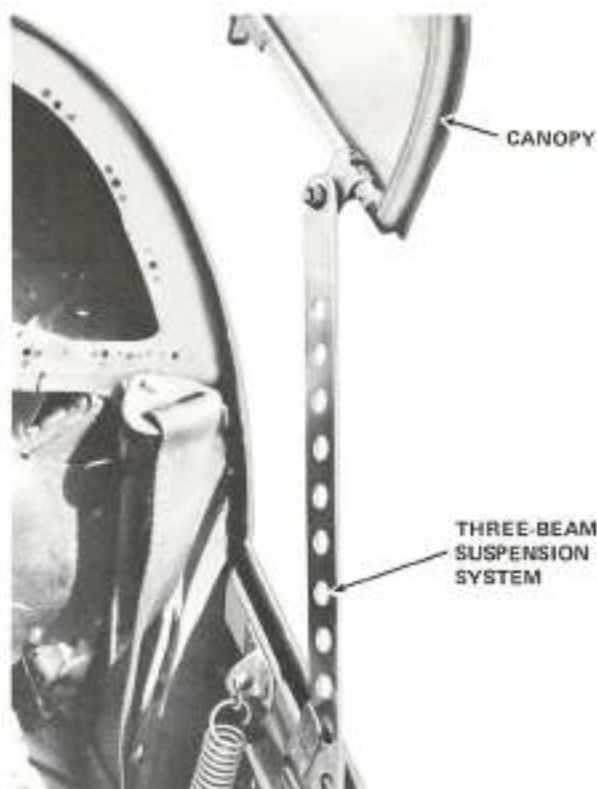
Figure 1-8 Canopy/Suspension System
