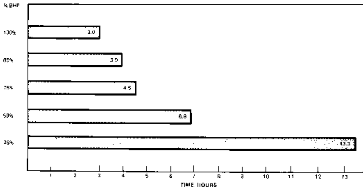
Figure A-7 Endurance Chart
