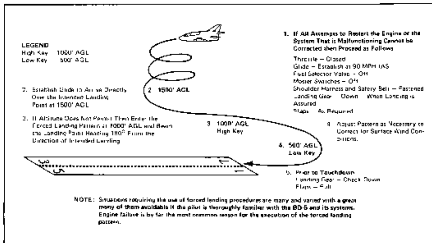
Figure 3-2 Diagram of Forced Landing Pattern
