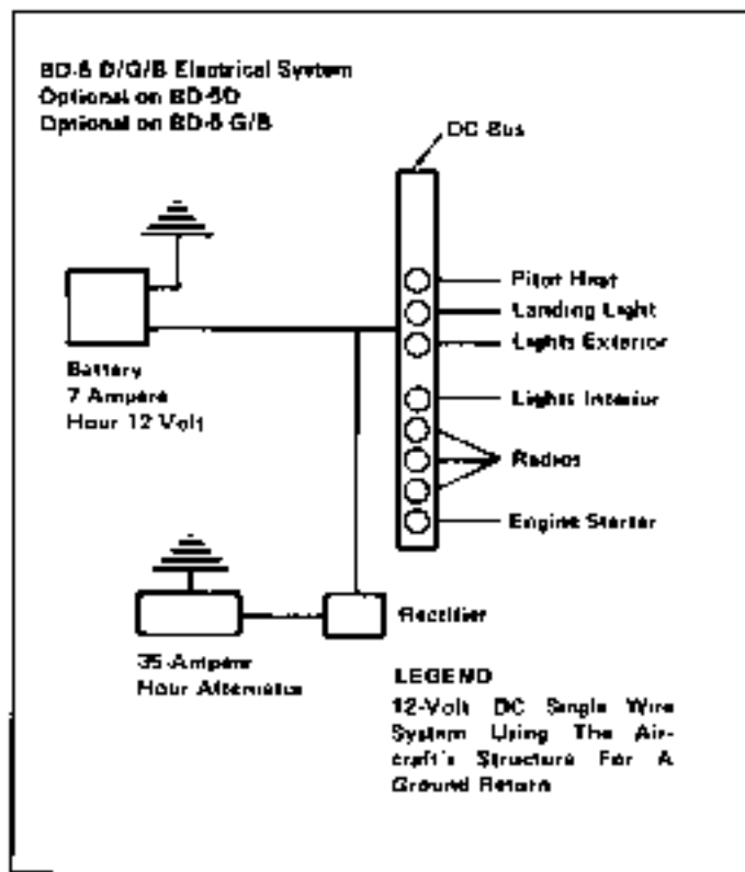
Figure 1-3 Electrical System
