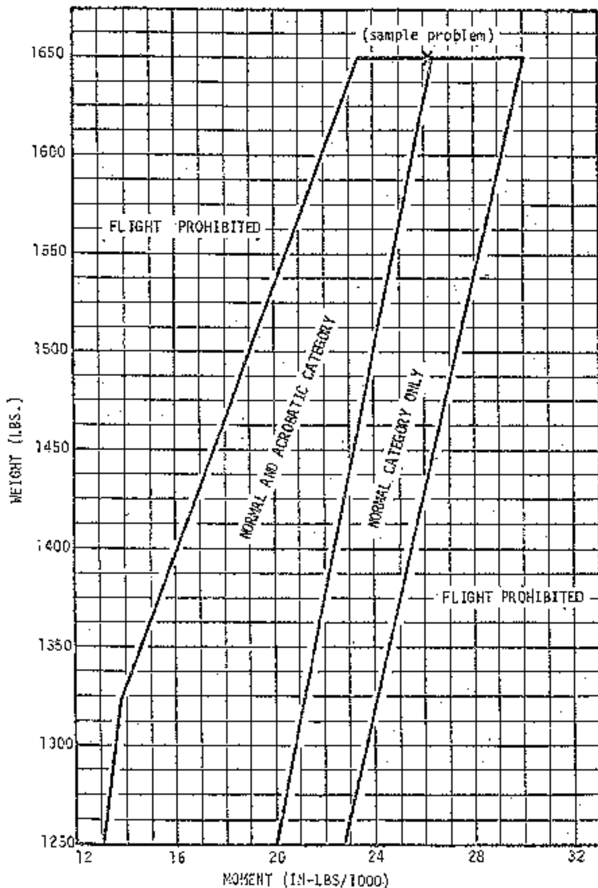
FIGURE 5-4 FLIGHT ENVELOPE - 790AR, 7K0AB ONLY
