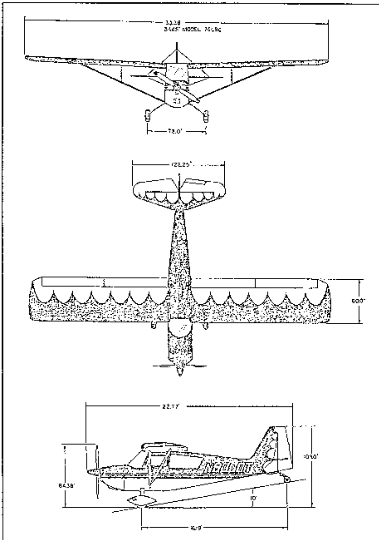
FIGURE 6-2 CITABRIA THREE-VIEW
