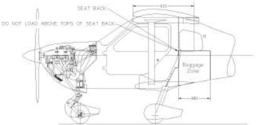
Figure 6.3.1 – Baggage Zones
